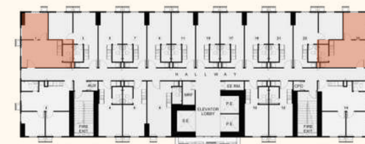
TYP. 4TH-21ST FLOOR PLAN
