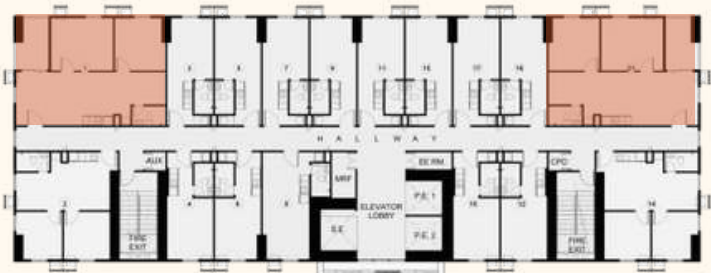
TYP. 22ND-23RD FLOOR PLAN
