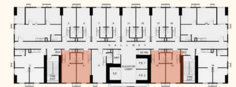
TYP. 22ND-23RD FLOOR PLAN
